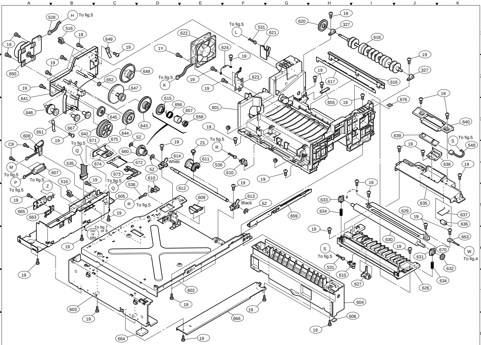
FIG. 6 PAPER TRANSPORTATION
