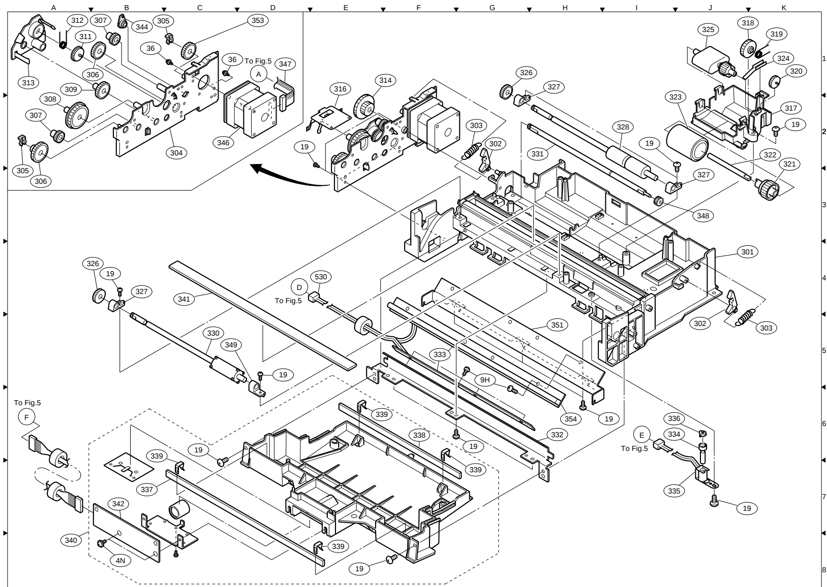
FIG. 3 TRANSMITTER ASSEMBLY
