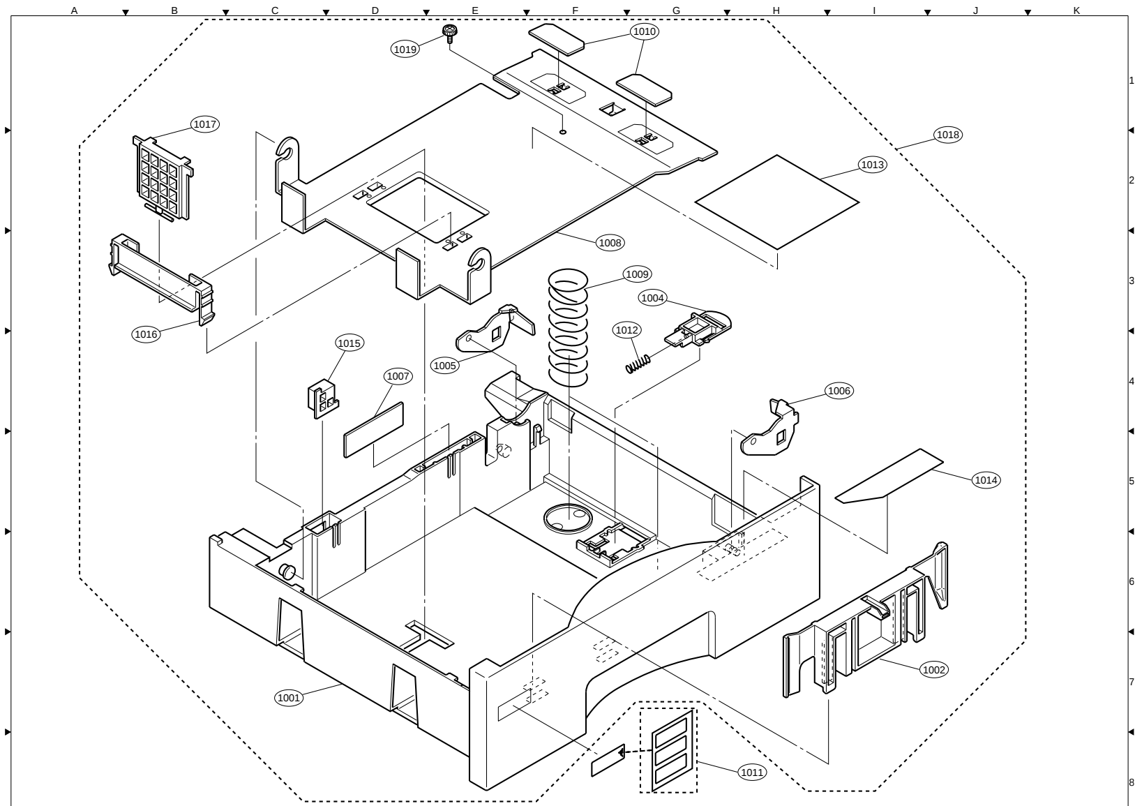
FIG. 10 500 PAPER CASSETTE
