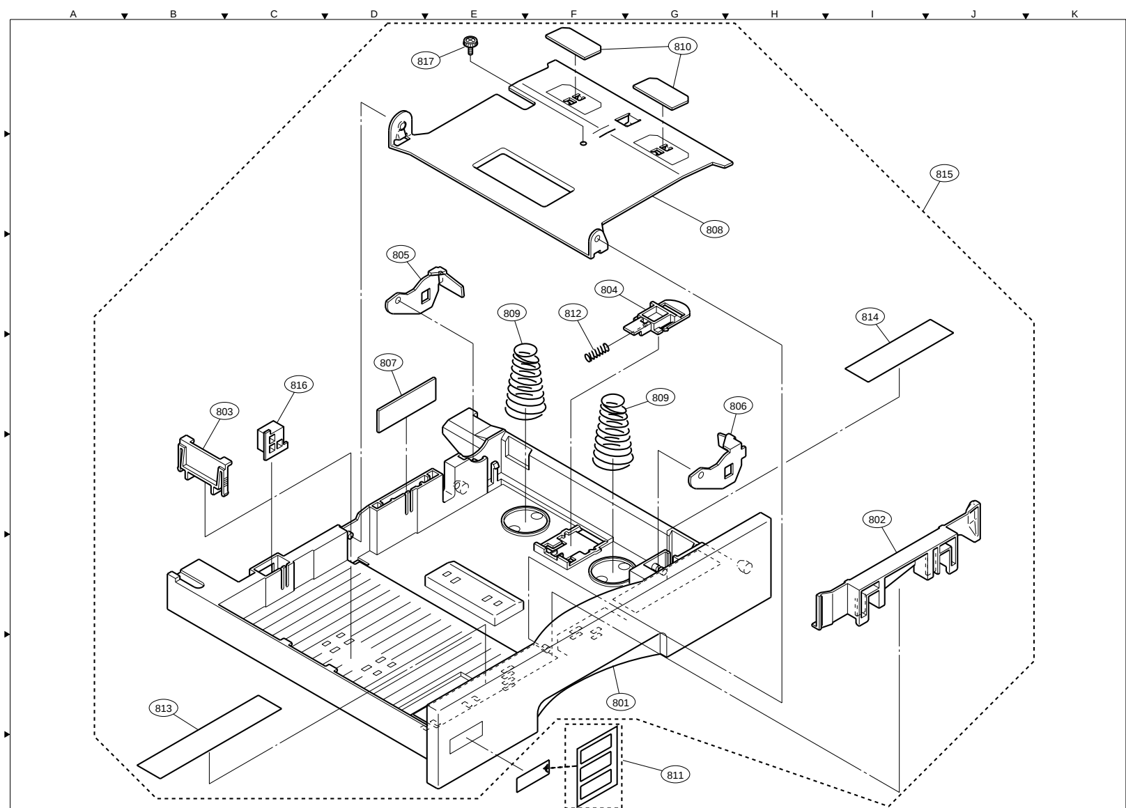
FIG. 8 250 PAPER CASSETTE
