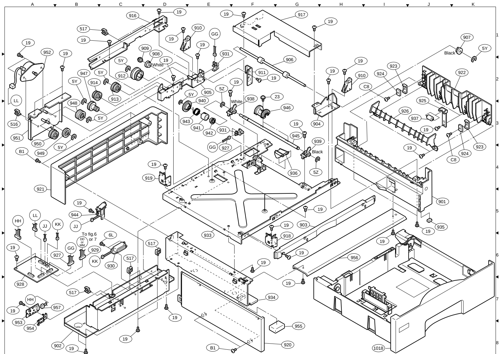
FIG. 9 500 FEEDER UNIT
